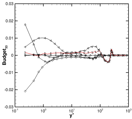
(e) \overline{\rho w'' w''} at (x - x_{imp})/\delta_{99} = -0.90
