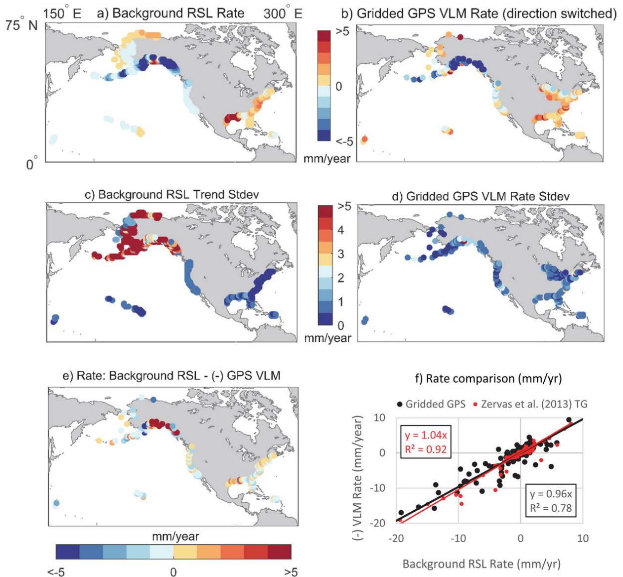
Figure 12. Gridded a) background RSL rates and b) GPS VLM rates (with directionality switched as to directly compare to RSL rate) with trend standard deviations shown in c) and d). In e) is the difference between the two rates shown in a) and b). In f) is a scatterplot and linear regression of the two sets of gridded rates shown in a) and b) as black dots and the red dots show background RSL rates as in a) but derived and compared to VLM estimated for more than 100 specific tide gauge (TG) locations used by Hall et al. (2016) and based upon Zervas et al. (2013).
