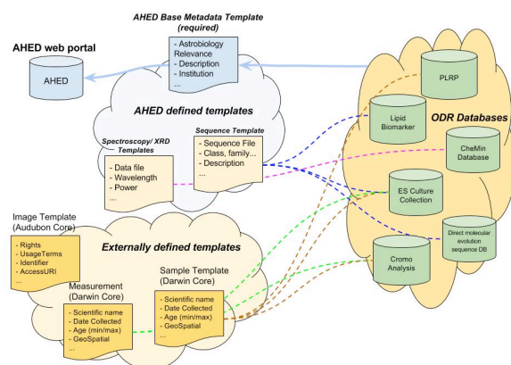
Figure 1. AHED framework of metadata templates.
