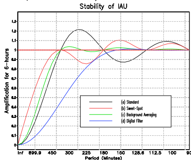
Above: Amplification factor for 6-hour IAU Corrector with difference strategies to avoid instability; traditional 3-hour Predictor shows as Standard (black curve).
