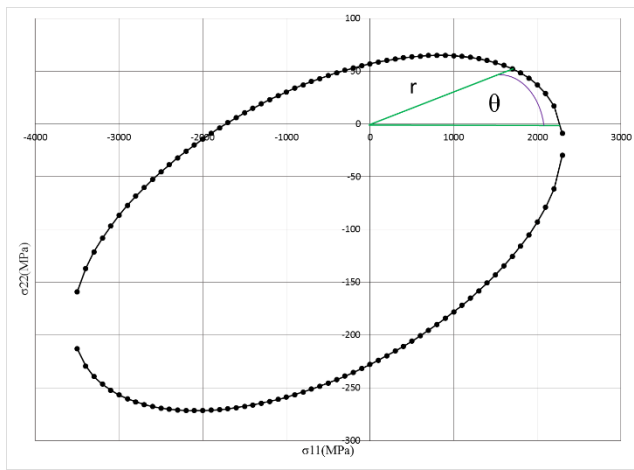
Figure 10. Tsai-Wu failure surface for AS4/3501-6 composite.
