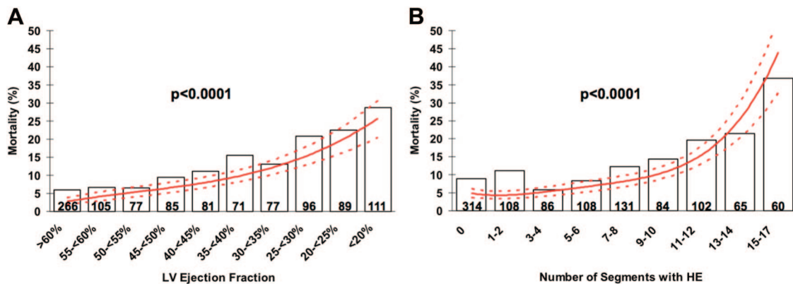
Figure 3. Mortality rate as a function of LVEF and amount of myocardial damage. The height of the bar and the number within represent the observed mortality rate at 2 years and total number of subjects for each category of LVEF (A) and HE (B). Solid lines represent Cox regression estimates (smoothed) of 2-year mortality adjusted for age and study site. Dashed lines represent 95% CIs. With each decrement in LVEF, there was a steadily increasing mortality rate. Likewise, increasing number of segments with HE was associated with higher mortality rates, although rates appeared to be similar in groups with ≤4 segments of HE. Abbreviations as in Figure 2.
