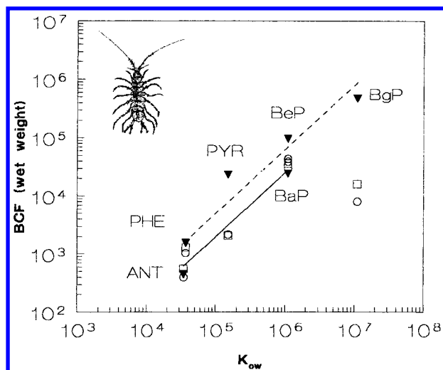
FIGURE 3. Rate constant-based two-compartment BCFs (wet weight, L kg -1 ; ▼) for theoretical equilibrium conditions ( t = \infty , according to eq 7), model-predicted BCFs at the end of the exposure period ( t = 7 days; ○), and measured apparent BCFs (mean values between days 3 and 7; □) in relation to n -octanol/water partitioning coefficients ( K_{ow} ; Table 1).
