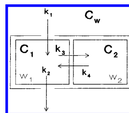
FIGURE 1. First-order rate constant two-compartment model applied in this study. Symbols and units are explained in the text.
