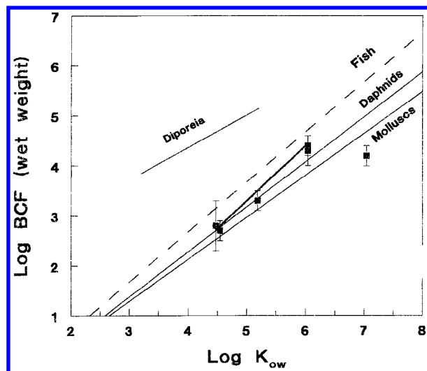
FIGURE 4. Apparent BCFs (log BCF; L kg -1 , wet weight; mean ± SE) for PAHs in freshwater isopods in relation to n -octanol/water partitioning coefficients (log K ow ) and similar linear relationships (solid lines; see Table 2) documented for fish (48), daphnids, mollusks (49), and a lipid-rich amphipod species (16, 65).
