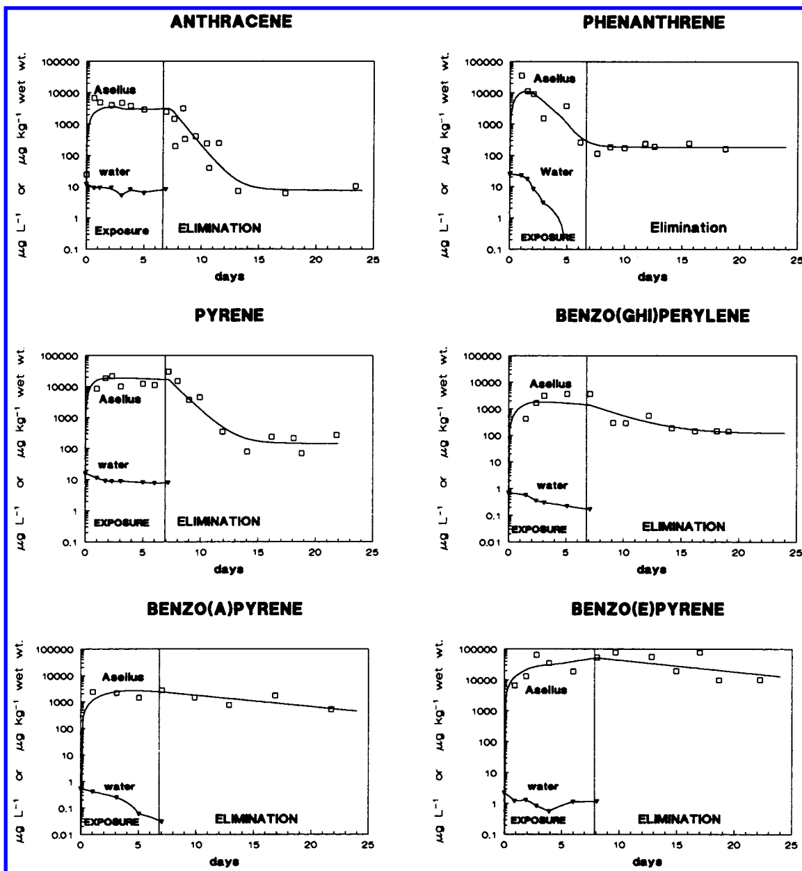
FIGURE 2. Bioconcentration and elimination of anthracene, phenanthrene, pyrene, benzo[ghi]perylene, benzo[a]pyrene, and benzo[e]pyrene in freshwater isopods in static exposure and depuration experiments: \square , mean wet weight concentrations in isopods ( \mu\text{g kg}^{-1} ); \blacktriangledown , aqueous concentrations ( \mu\text{g L}^{-1} ). The solid lines indicate the model predictions for the whole body concentrations and the linearly interpolated water concentrations.
