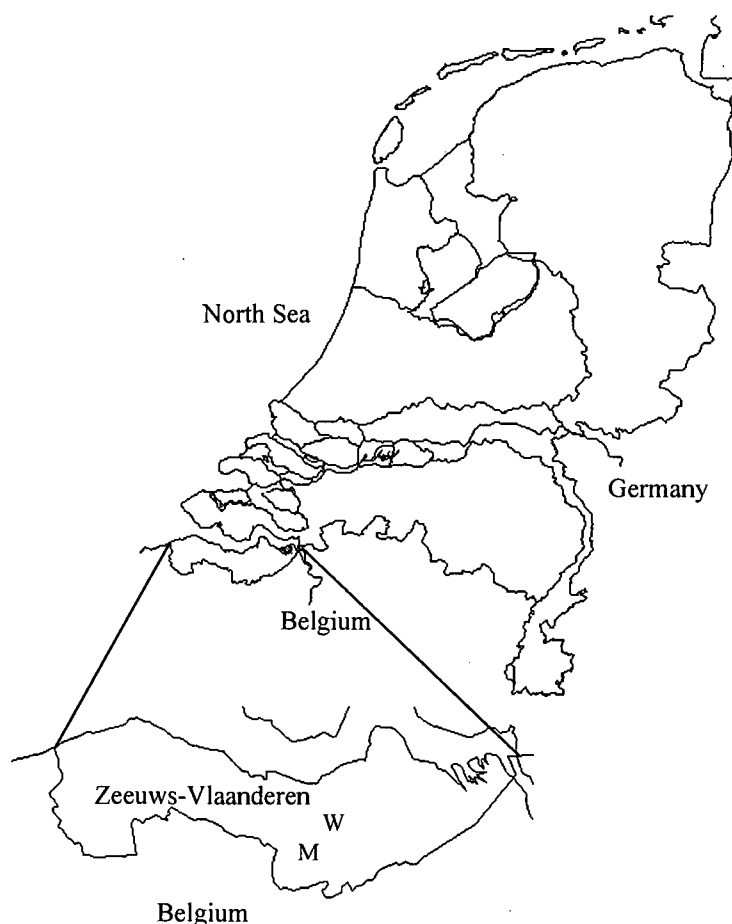
Figure 1. The Netherlands and an Enlargement of Zeeuws-Vlaanderen (W = Case Waterspil; M = Case Moerspui).
