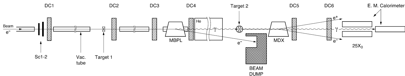
Fig. 1. A schematical drawing of the setup used in the experiment. The total length of the setup is about 65 m.
