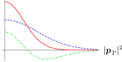
Fig. 2. Possible behavior of the universal distribution function f_1(x, p_T^2) (dashed line) and the process-dependent function f_1^{(ab \rightarrow cd)}(x, p_T^2) (solid line) as a function of |p_T|^2 . Their difference-function, \delta f_1^{(ab \rightarrow cd)}(x, p_T^2) (dash-dotted line), vanishes upon integration over p_T .
