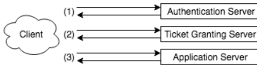
Figure 2.5: Kerberos as standardized in [MNSS88]. (1) is called the AS-exchange; (2) the TGS-exchange; and (3) the AP-exchange
