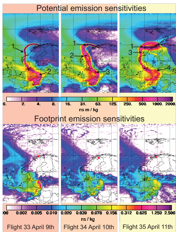
Fig. 2. FLEXPART column-integrated potential emission sensitivities (PES, top) and footprint emission sensitivities (FPES, bottom) for the anthropogenic air mass sampled during the flights on 9, 10 and 11 April 2008. Numbers indicate the air mass age in days at the location pointed by corresponding black arrows. On FES maps, red squares indicate the aircraft location, used as a starting point to run FLEXPART.
