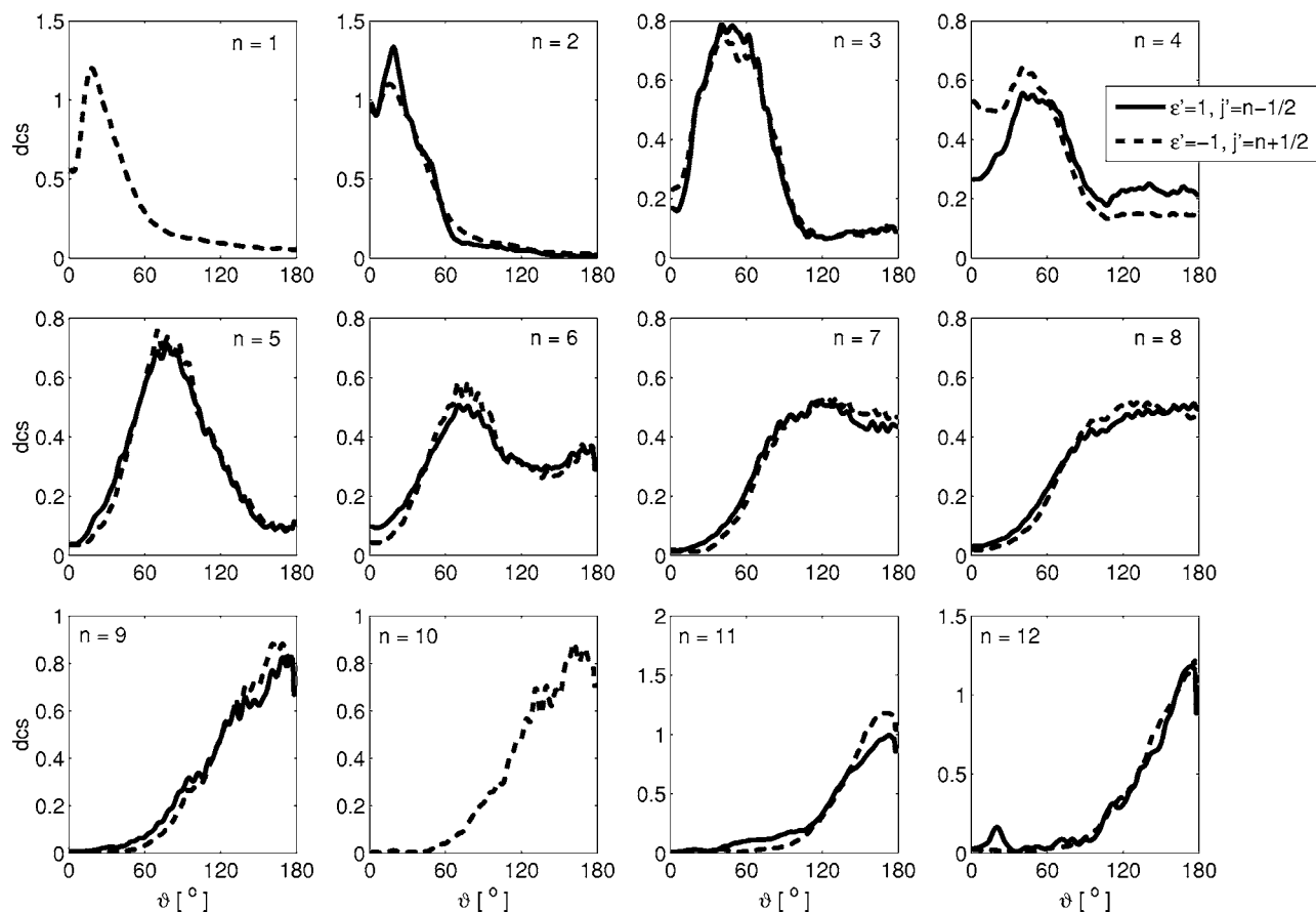
FIG. 6. Differential cross sections for (He-NO) scattering into \Omega' = 1/2 . The differential cross sections are plotted per parity pair and normalized such that the integral \int d\vartheta d\sigma = 1 .
