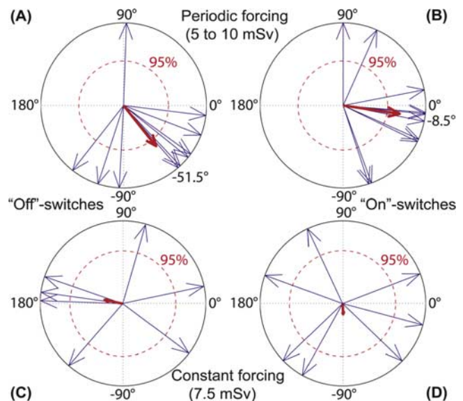
Figure 3. Statistical significance of the phase locking between the periodic forcing and the state-transitions in overturning circulation. The timing of the “off”- and “on”-switches relative to the phase of the forcing can be mapped as vectors in a unit circle (see Figure 2 (insets) and auxiliary material). For random timing of the transitions, the lengths of the averaged vectors (bold arrows) would tend to zero. In the (top) periodically forced run the average vectors of both (left) the “off”-switches and (right) the “on”-switches exceed a critical length (dashed circles), indicating a significant ( p < 0.05 , n = 10 ) phase locking between the periodic forcing and the timing of the events. In the (bottom) control experiment with 7.5 mSv constant forcing (see Figure 1b) the lengths of the mean vectors stay well below the significance level, indicating that the timing of the state-switches cannot be predicted.
