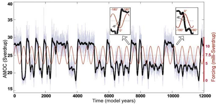
Figure 2. State transitions in Atlantic meridional overturning circulation (AMOC) with periodic freshwater forcing in the Labrador Sea. The 73-year running mean (black) of the AMOC (light blue) shows multicentennial state transitions. The superimposed sine function (red) represents the external small periodic freshwater forcing in the Labrador Sea (note 1000 times amplified, scale on the right). The absolute timing of a state switch is defined as the model-year in which the running mean of the Atlantic meridional overturning circulation crosses the 25 Sv line (dashed). The state switches, associated with “on” and “off” modes in Labrador Sea convection, follow the beat of the forcing, but sometimes beats are skipped. In order to evaluate whether this phase locking is statistically significant (Figure 3), the relative timing of each “off”-switch is defined as a phase difference with the nearest forcing-maximum. (right inset) For example, the event at year 10,116 has a phase lag of -6^\circ with the forcing that peaks at year 10,125 ( (-9 \text{ yr}/500 \text{ yr}) \times 360^\circ ). (left inset) Likewise the timing of each “on”-switch is defined as a phase difference with the nearest forcing-minimum (see auxiliary material for details).
