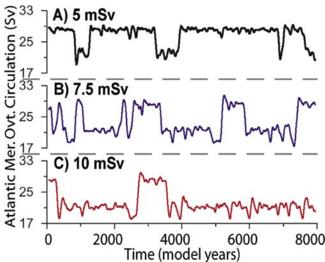
Figure 1. A constant Labrador Sea freshwater forcing of 5 mSv, 7.5 mSv, and 10 mSv, respectively, pushes the Atlantic meridional overturning circulation (AMOC) into a bistable regime, leading to random switches between a strong (29 Sv) and a weak (21 Sv) state. The weak state is associated with lack of convection in the Labrador Sea [cf. Schulz et al. , 2007, Figure 2]. With increasing magnitude of the freshwater forcing, the probability for the system to occupy the weak state rises, but apparently the system remains in the deterministically bistable regime over the whole range of applied forcings. (The time series shown are smoothed with a 101-year Hanning filter).
