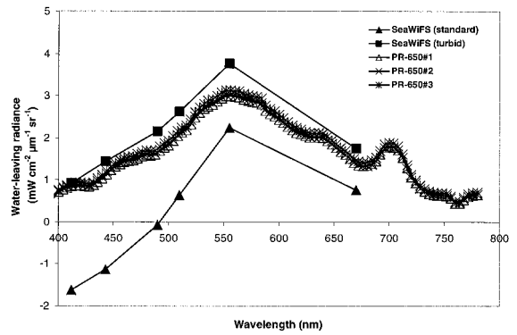
Fig. 8. Comparison of in situ PR-650 colorimeter measurements of water-leaving radiance for Lake Markermeer taken on 25 June 1999 at 12:48 UTC with coincident spectra from the SeaWiFS image acquired at 11:31 UTC and processed with the standard and the new turbid water atmospheric correction algorithms.
