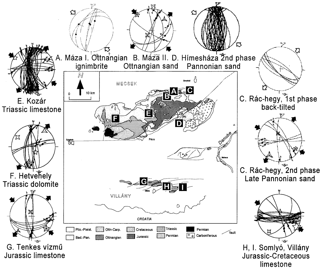
Fig. 7. Structural data from SW Hungary, indicating NW-SE shortening, NE-SW elongation. Data taken from Bergerat and Csontos (1984), Csontos and Bergerat (1993), Benkovics (1997). Measured outcrops indicated by dot and Capital. All stereo-plots in lower hemisphere Schmidt projection. Fault is indicated by trace, striae by dot; small arrows indicate observed offset. Outer large arrows indicate compression and extension directions. Empty arrows indicate stress directions inferred from observed structures. Star, Triangle and Diamonds stand for computed \sigma_1 , \sigma_3 , \sigma_2 directions, respectively. Extension directions in outcrop C, first phase, are inferred after back-tilting by measured bedding dip value.
