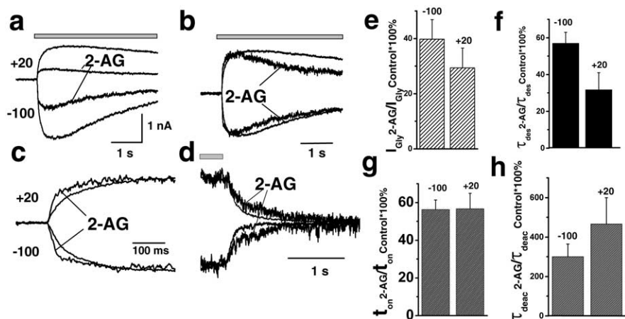
Figure 3. Voltage dependence of the I_{\text{Gly}} modulation by 2-AG. a , Representative traces obtained in control condition and in the presence of 1 \mu\text{M} 2-AG at holding potentials of -100 and +20 mV. b, c , Corresponding traces normalized and superimposed. d , Deactivation of I_{\text{Gly}} before and after preapplication with 2-AG. e-h , Statistics for the 2-AG effects on peak amplitude ( e ), \tau_{\text{des}} ( f ), t_{\text{on}} ( g ), and \tau_{\text{deac}} ( h ) obtained at holding potentials of -100 and +20 mV.
