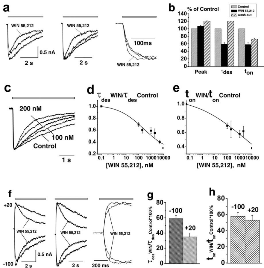
Figure 4. Modulation of glycine-activated currents by WIN 55,212-2. a , Left, Traces of I_{\text{Gly}} induced by 100 \mu\text{M} Gly obtained in control, in the presence of WIN 55,212-2 ( 1 \mu\text{M} ), and after washout of drug (gray line) ( V_h = -100 mV). Middle and right, The same traces are superimposed and normalized. b , Statistics of the effects of WIN 55,212-2 on the amplitude, \tau_{\text{des}} , and t_{\text{on}} ( n = 11 ) of I_{\text{Gly}} . c-e , Concentration dependence of the WIN 55,212-2 effects on I_{\text{Gly}} kinetics. c , I_{\text{Gly}} traces recorded at various concentration of WIN 55,212-2 ranged from 100 nM to 2 \mu\text{M} measured in the same cell are normalized and superimposed. d, e , Summary plots showing the effect of increasing the WIN 55,212-2 concentrations on \tau_{\text{des}} ( d ) and t_{\text{on}} ( e ) measured at V_h = -100 mV ( n = 4 ). Data are plotted as a fraction of the maximal glycine current in control. f-h , Voltage dependence of the I_{\text{Gly}} modulation by the WIN 55,212-2. f , Left, I_{\text{Gly}} representative traces obtained in control condition and in the presence of 1 \mu\text{M} WIN 55,212-2 at holding potentials of -100 mV and +20 mV. Middle and right, The same traces are superimposed and normalized. Statistics for the WIN 55,212-2 effects on \tau_{\text{des}} ( g ) and t_{\text{on}} ( h ) at holding voltages of -100 and +20 mV.
