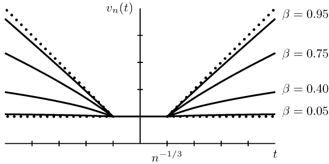
FIG. 2. Plot of v_n(t) for various values of \beta . The dotted lines are y = t and y = n^{-1/3} . Note that \beta close to zero gives the sharpest bound.
