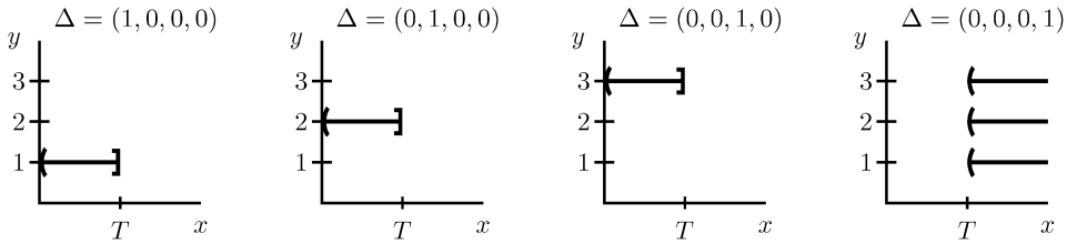
FIG. 1. Graphical representation of the observed data (T, \Delta) in an example with K = 3 competing risks. The black sets indicate the values of (X, Y) that are consistent with (T, \Delta) , for each of the four possible values of \Delta .
