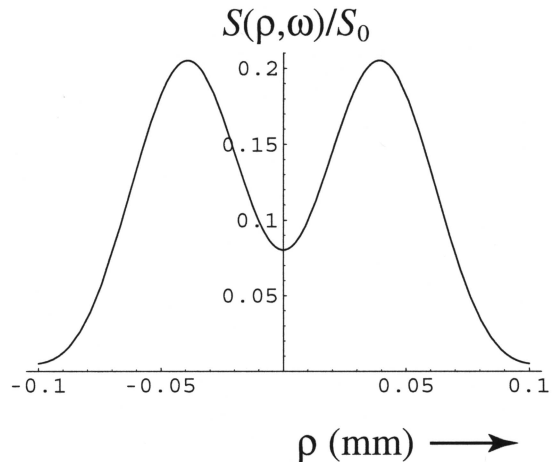
Fig. 3. Intensity in the focal plane for 1/\beta = 3.53 mm, showing a local minimum at focus. All other parameters are as in Fig. 2.
