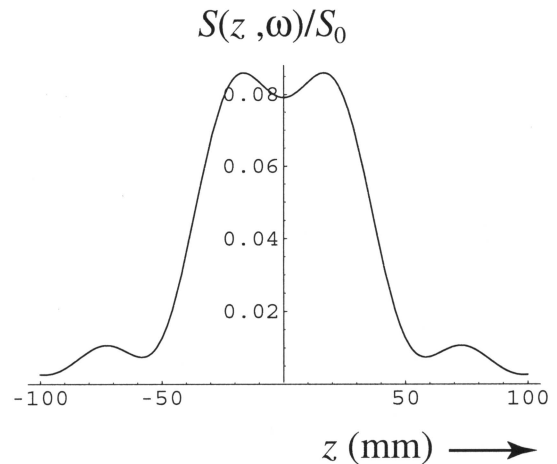
Fig. 2. On-axis intensity distribution for 1/\beta = 3.53 mm, showing a local minimum at focus, with a = 10 mm, f = 2 m, and \lambda = 500 nm.
