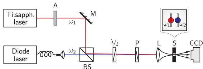
Fig. 1. (Color online) Sketch of the experimental setup. The outputs of a fiber-coupled diode and a Ti:sapphire laser are individually focused on one of a pair of 200 nm wide slits, separated by \approx 25 \mu\text{m} , in a thin gold film. The light diffracted at the two parallel slits is imaged onto a CCD camera. A, attenuator; M, mirror; BS, beam splitter; \lambda/2 , half-wave plate; P, polarizer; L, lens; S, gold sample. The inset shows the illumination of the double slit.
