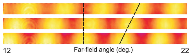
Fig. 3. (Color online) Interference patterns recorded with only a single slit illuminated by the TM-polarized output of the Ti:sapphire laser for, from top to bottom, \lambda = 767 \text{ nm} , \lambda = 775 \text{ nm} , and \lambda = 784 \text{ nm} .
