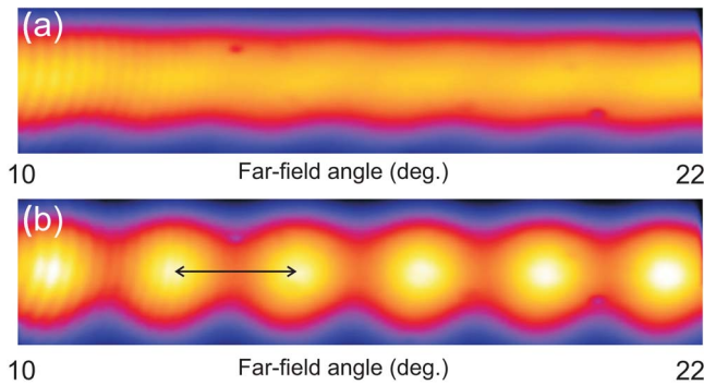
Fig. 2. (Color online) (a) Far-field pattern for the case when both laser beams are TE-polarized (polarization parallel to the slits). The semiconductor laser emits at 812 nm, while the Ti:sapphire laser is tuned to 808 nm. (b) Experimental far-field pattern when the polarization of both laser beams is perpendicular to the two slits (TM-polarization). Large-period fringes with a visibility \mathcal{V} \approx 20\% are easily discerned. The arrow indicates the period of the fringes.
