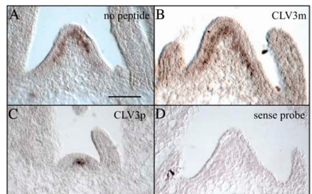
Figure 5. WUS expression in clv3-2 upon incubation with CLV3p. A to C, In situ hybridization using an antisense probe of WUS cDNA showing the WUS expression in the SAM of clv3-2 after 8 d of treatment. Treatment with no peptide (A) or CLV3m (B) resulted in an expanded WUS expression as compared to clv3-2 treated with CLV3p (C) in which the WUS expression is restricted to the OC as seen in wild type. D, Control sample treated with CLV3m and hybridized with the WUS sense probe. The bar in A represents 50 \mu\text{m} for all samples.
