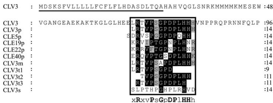
Figure 1. Alignment of CLV3 and the synthetic peptides used for the in vitro assay. Identical amino acids are shaded in black and similar ones in gray, the signal sequences are underlined, and the CLE box is framed with the consensus sequence underneath.
