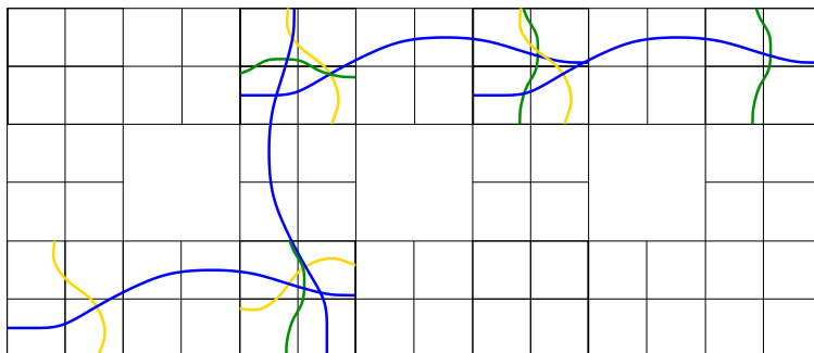
Figure 2: The event depicted above and its rotation by 90 degrees can be used to couple the complement of the soup to a one-dependent percolation process on a square grid whose open edges correspond to rectangles where the event occurs. We denote by p_n the probability of the event when the elementary squares in the figure have side length 3^n , i.e., the probability that an edge is open in the corresponding bond percolation process. (As in Fig. 1, the different colors for the crossings serve only to enhance the visibility of the figure.)
