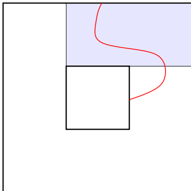
Figure 4: The shaded rectangle is crossed in the “easy” direction.
