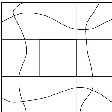
Figure 3: Four crossings of rectangles forming a circuit inside an annulus.
