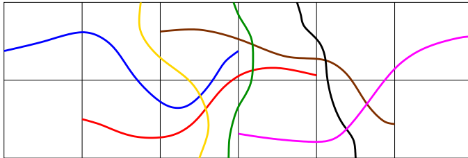
Figure 1: Pasting horizontal crossings of 3 by 2 rectangles and vertical crossings of 2 by 2 squares, a crossing of a 6 by 2 rectangle is obtained. (The different colors for the crossings serve only to enhance the visibility of the figure.)
