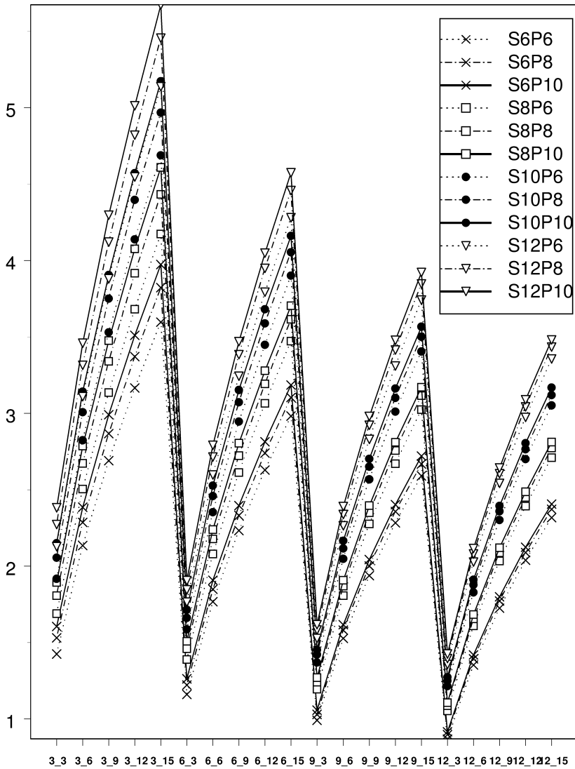
Figure 2. Z-scores for \sigma_7^2 as a function of component values and number of factor levels.
