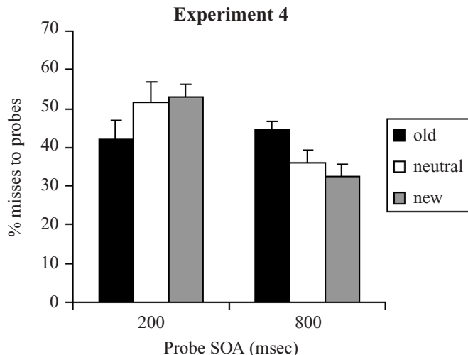
Figure 10. Percentages of misses to probes in Experiment 4 (preview search, stimulus onset asynchronies [SOAs] of 200 and 800 msec). Bars indicate the standard errors.
