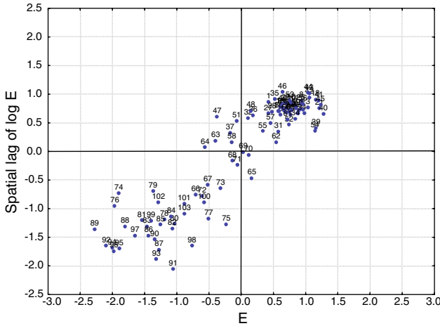
Fig. 2 Moran scatterplot of E
