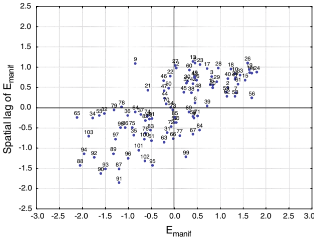
Fig. 4 Moran scatterplot of E_{manif}
