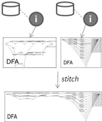
Figure 3. Complementary learning
