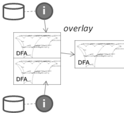
Figure 4. Congruent learning
