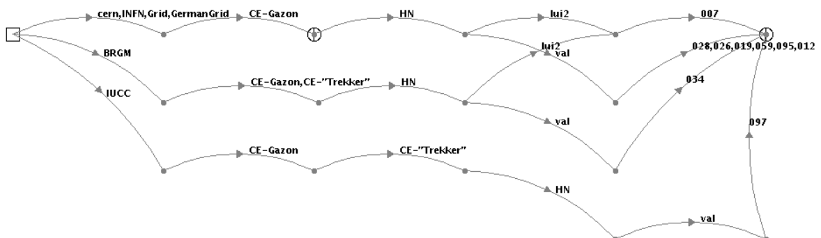
Figure 6. Resubmitted job traffic DFA graph.
