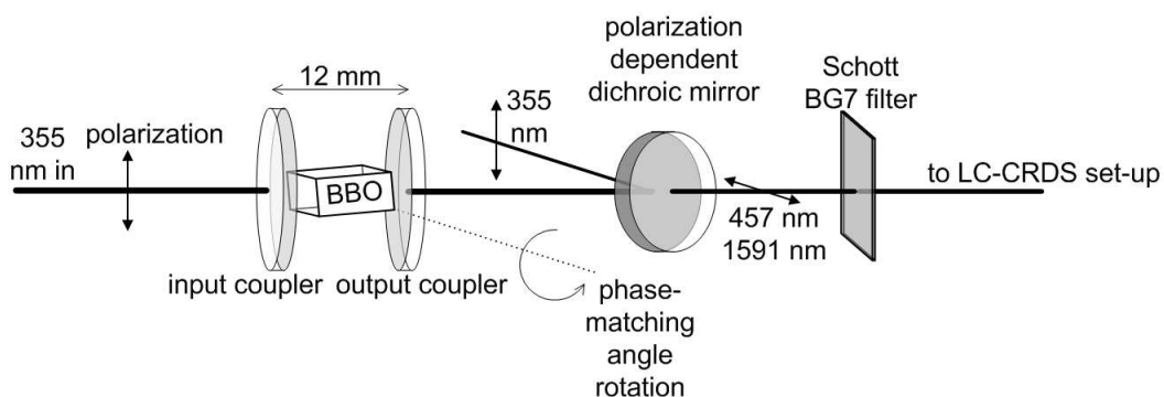
Figure 4.3: Schematic diagram of the wavelength-tunable OPO laser light source delivering laser pulses in the range 425 - 475 nm at a bandwidth of around 0.2 nm.
