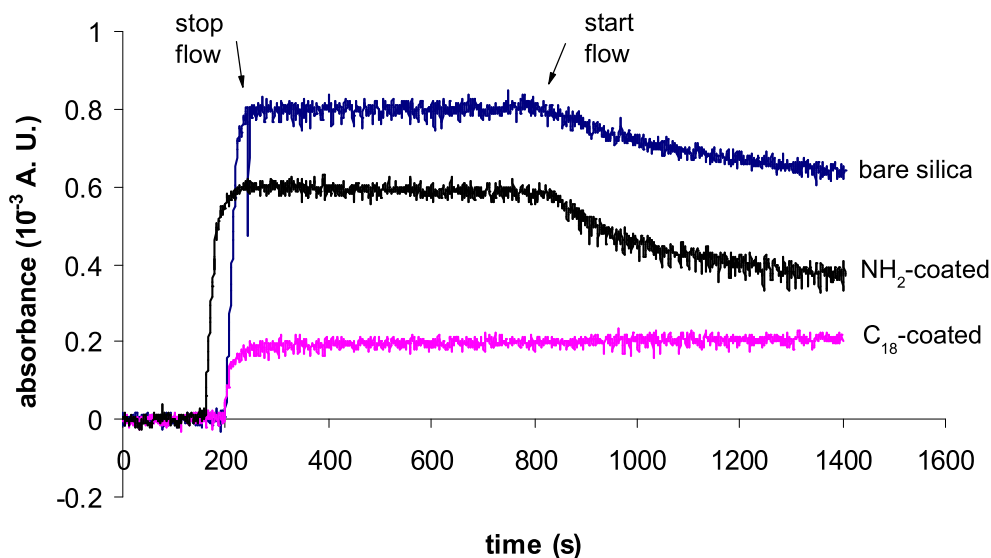
Figure 7.3: Flow profiles on the different surfaces; cyt c concentration: 10 \mu\text{M} . From top to bottom: the bare silica surface, the \text{NH}_2 -coated surface and the \text{C}_{18} -coated surface.
