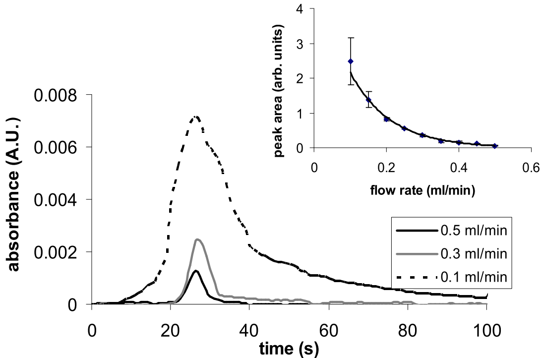
Figure 6.4: Influence of flow rate on CV adsorption. Flow profiles showing an injection of 20 \mu\text{M} of CV in 10 \text{ mM} potassium phosphate buffer, \text{pH} = 7.4 on the super-polished TIR surface. Flow rates are 0.1 , 0.3 and 0.5 \text{ ml/min} , sample injection volume 100 \mu\text{l} . Profiles were horizontally shifted for ease of comparison. The values on the y-axis are in absorbance units. The inset shows the peak area as a function of flow rate as measured for 20 \mu\text{M} of CV on the standard polished TIR surface.
