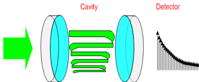
Figure 1.1: Schematics of the principle of CRDS. After abrupt termination of the excitation, the light stored in the cavity will decay exponentially as it bounces back and forth between the mirrors losing a small portion at each reflection. The decay rate of this light can be measured behind the cavity.
