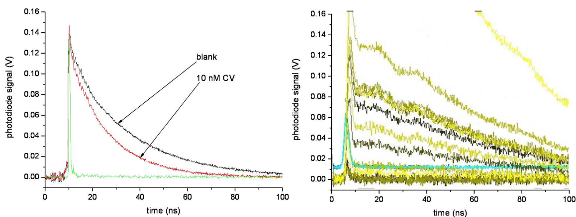
Figure 1.4: Ring-down curves as taken under pulsed multi-mode conditions are shown to the left. Each laser shot is able to excite many modes in the cavity, this is the desired situation. An instrumental response function is shown together with a ring-down curve of a methanol-filled cavity and one with absorber (10 nM Crystal Violet). The cavity was a 2-mm liquid-only cavity; the complete experiment is described in chapter 2 [27]. Since the 2-mm cavity has a large FSR, mode-beating effects can readily be observed for narrow-band lasers (to the right, the experiment is the same except for the use of a Fourier-transform limited laser). As the length of the cavity fluctuates due to ambient temperature drifts, the laser might or might not excite the cavity and one might or might not observe a ring-down.
