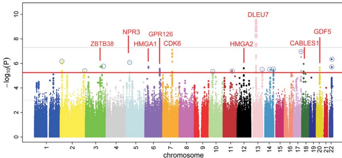
Figure 1. Manhattan plot of the height association test results ( \log_{10}(P) ) for all SNPs in the stage 1 data set ( n = 10\,074 ). Red and grey lines are the suggestive ( 5 \times 10^{-6} ) and genome-wide significance ( 5 \times 10^{-8} ) P -value thresholds, respectively. Signals passing the suggestive threshold, and with the respective gene name given in red, are previously known regions of height association. Twelve loci for which SNPs were selected for the stage 2 analyses are emphasized by a blue circle.
