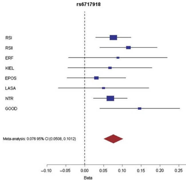
Figure 4. Forrest plot for the most significant SNP (rs6717918) in the combined meta-analysis of both the stage 1 and the stage 2 data sets. Beta: increase in height per SNP allele. Blue squares represent effect size estimates (measured in standard deviations of height) and 95% CI for each study. The red diamond represents the summary effect size estimate.
