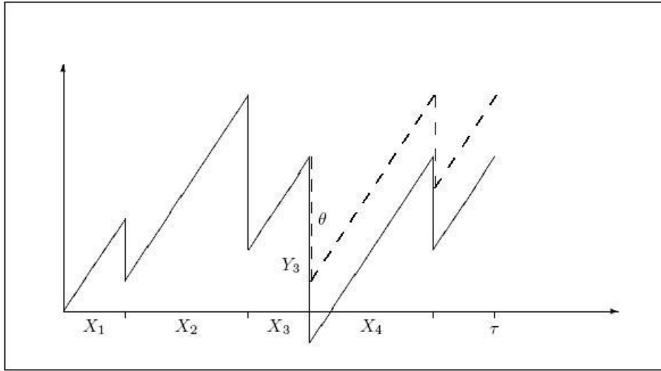
Figure 3: An occurrence of the event \mathfrak{R}_\tau \setminus \mathfrak{R}_\tau^3 and N_\tau = 4 . The dashed line represents a version of the process where the value of the 3^{rd} claim is reduced.
