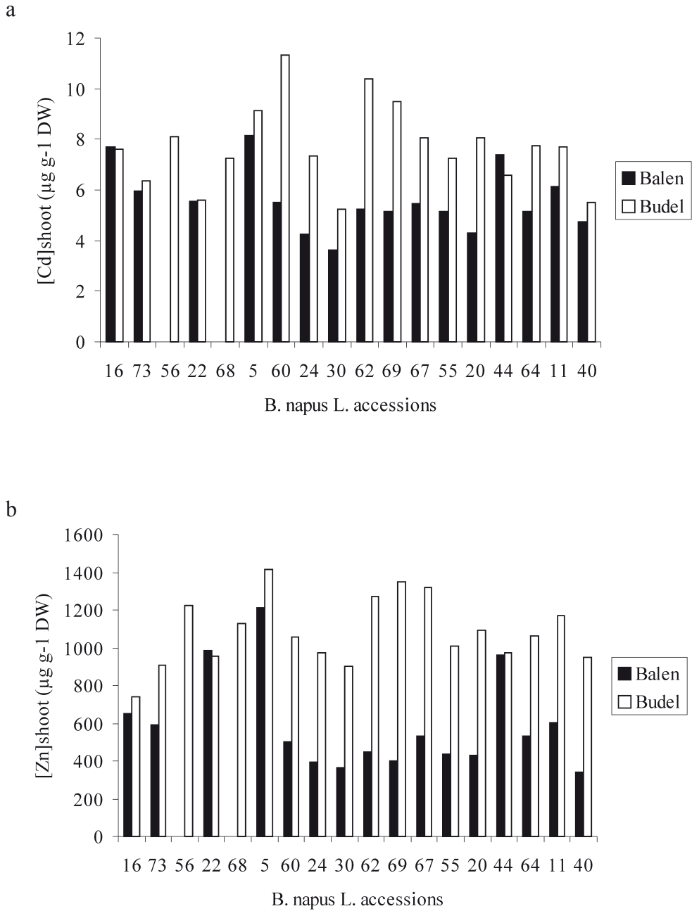
Figure 2. (a) [Cd]shoot ( \mu\text{g g}^{-1} DW) of the B. napus L. accessions (n=4) in Budel and Balen. (b) [Zn]shoot ( \mu\text{g g}^{-1} DW) of the B. napus L. accessions (n=4) in Budel and Balen.
