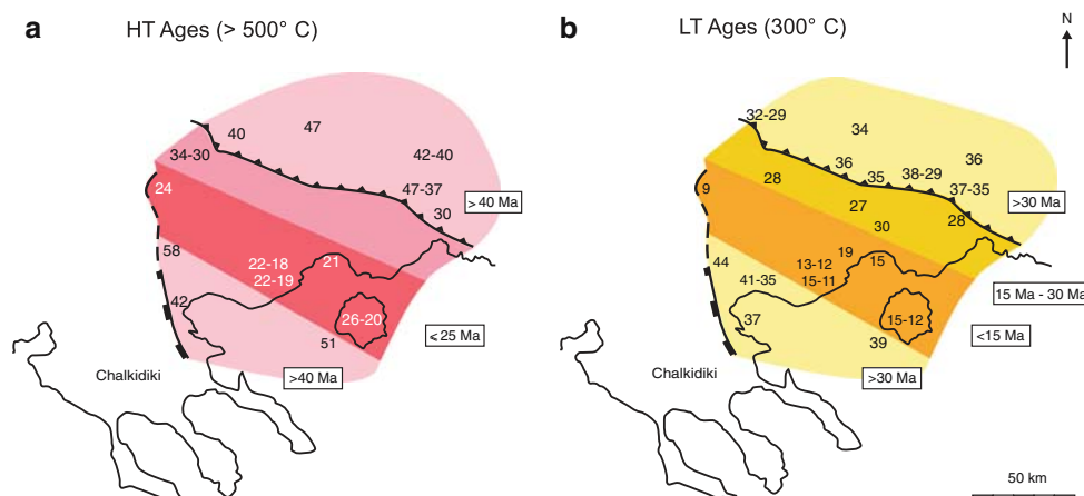
Fig. 2 Geochronological ages in the Southern Rhodope Core Complex for closing temperatures of 500°C or higher (a) and of 300°C (b). In both diagrams, the darker band corresponds to the youngest ages in the inner SRCC. Data from Del Moro et al. (1990), Dinter (1998), Dinter et al. (1995), Harkovska (1983), Harre et al.
