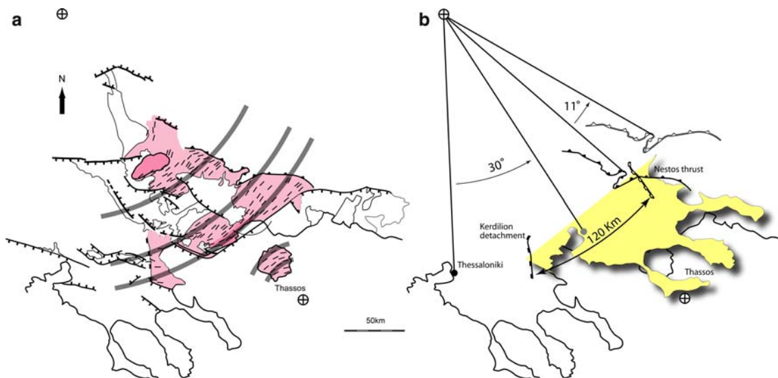
Fig. 18 Restoration of block rotation at the scale of the Southern Rhodope Core Complex. a Determination of the poles of rotation from the stretching lineation pattern. b Restoration of block rotation, taking into account the available paleomagnetic data with, in particular, mean dextral rotations of 30^\circ for the Chalkidiki and 11^\circ
