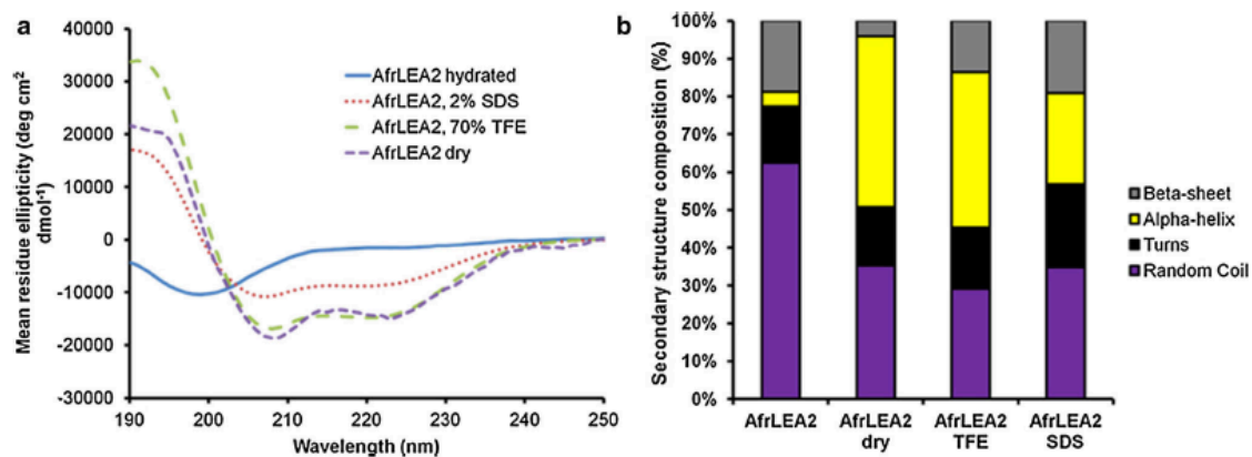
Fig. 2 Left panel CD spectra for recombinant AfrLEA2 in the hydrated state, in the presence of 2 % SDS, 70 % TFE, and after desiccation. Right panel secondary structure composition of recombinant AfrLEA2 for the above conditions, as calculated from the respective CD data with appropriate algorithms (adapted from Boswell et al. 2014b)
