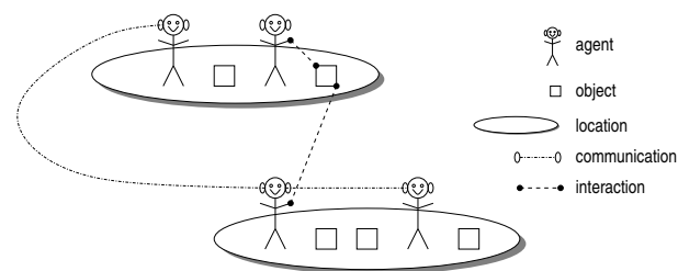
Figure 1: AgentScape conceptual model.
