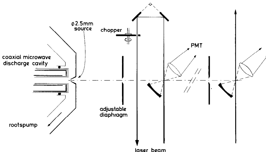
Fig. 1. Scheme of the experimental arrangement.
