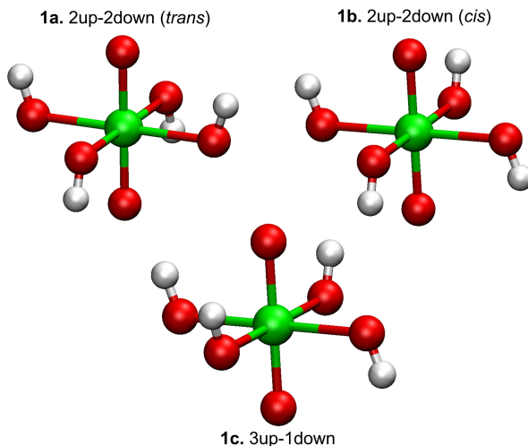
Figure 7.1: Three local minima of tetrahydroxouranilate: the trans (top-left), cis (top-right) and 3up-1down conformations. The trans conformer is the most stable.
