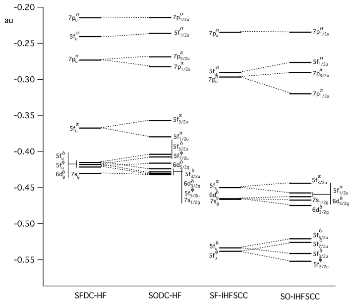
Figure 4.1: The energy affinities of the 5f , 7s , 6d and 7p orbitals have been sketched for the \text{UO}_2^{2+} molecule. On the left, the spin-free and spin-orbit coupling contributions calculated at DC-HF level. On the right, the more accurate values from sector (0,1) of the IHFSCC calculations are given. The correlated space for dynamical energy was (24e/6au), while the P model space was (17g,20u) with 7p 's orbitals included in the P_m . All these calculations were performed with the Faegri basis set. The bond distance is 1.770 Å.
