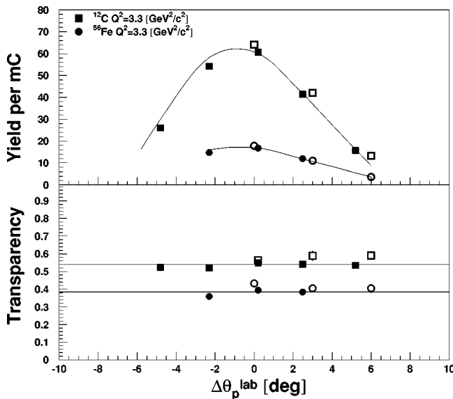
FIG. 3. (Upper panel) Experimental (e, e'p) coincidence yields versus the difference between the proton spectrometer lab angle and the quasifree angle for data from ^{12}\text{C}(e, e'p) and ^{56}\text{Fe}(e, e'p) at Q^2 = 3.3 ( \text{GeV}/c ) ^2 . Closed symbols are for the present experiment. Open symbols are for the data from Ref. [16]. (Lower panel) Transparency as function of proton angle for the same data. The curves in the top panel are simulations of the yield based on the model described in the text and normalized by a single transparency factor.
