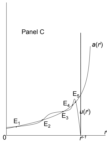
Figure 2. Equilibria
