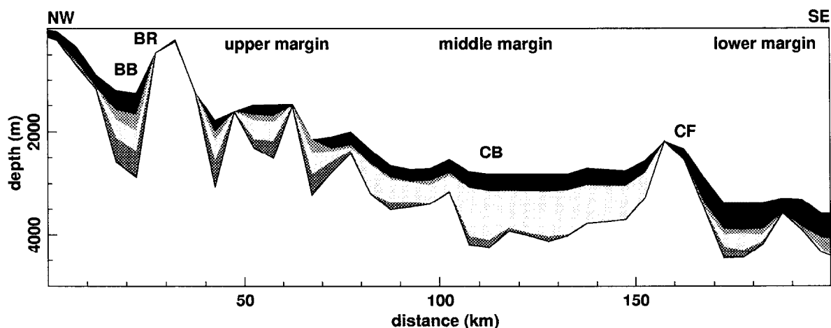
Fig. 10. Predicted stratigraphy for a 4-Ma post-rift phase. Post-rift sedimentary unit in black. Considering a longer post-rift phase (break-up at 4 Ma) we obtain a surplus of post-rift sediments in comparison to the observed record (Fig. 2). In order to obtain a good fit with the observed stratigraphy the water depth at the end of rifting can be decreased: in this case the predicted deepening of the basin during the post-rift phase reaches values around 400–500 m. BB = Baronic basin, BR = Baronic ridge, CB = Cornaglia basin, CF = Central Fault.
