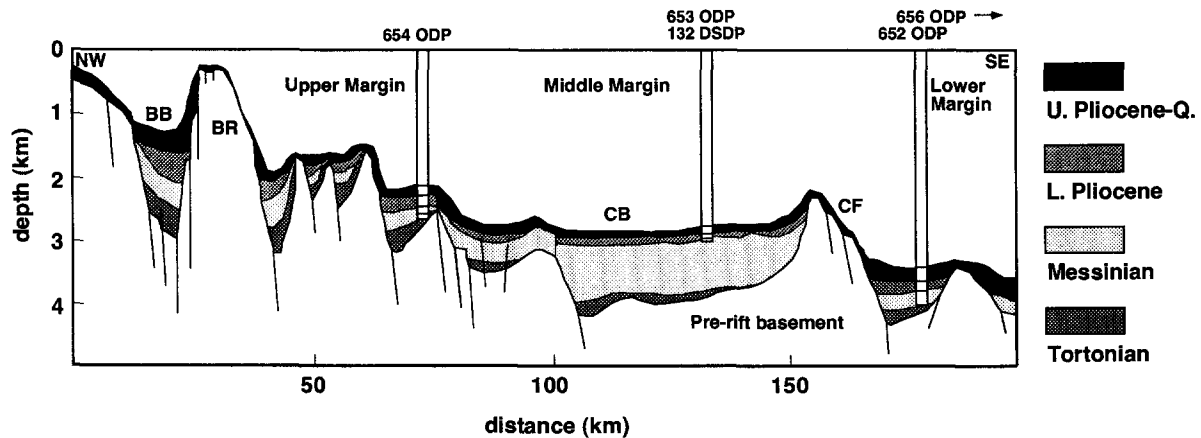
Fig. 2. Section A–B (Fig. 1). Observed stratigraphy along the Sardinian passive continental margin. Projections of the ODP and DSDP boreholes are shown. The section is based on Mascle and Rehault (1990), Bartole (1981) and references therein. Time/depth conversion was made according to interval velocities measurements at drilled sites (ODP Leg 107) and to multi-channel seismic profiles information. BB = Baronic basin, BR = Baronic ridge, CB = Cornaglia basin, CF = Central Fault.
