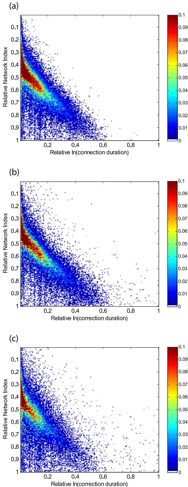
Figure 5. The relationship between the RNI and the logarithm of connection duration scaled by the maximum modeled connection time. This is shown as a two-dimensional probability density function with 0.05 width probability bins. (a) The full catchment and the (b) eastern and (c) western subcatchments (see Figure 2).
