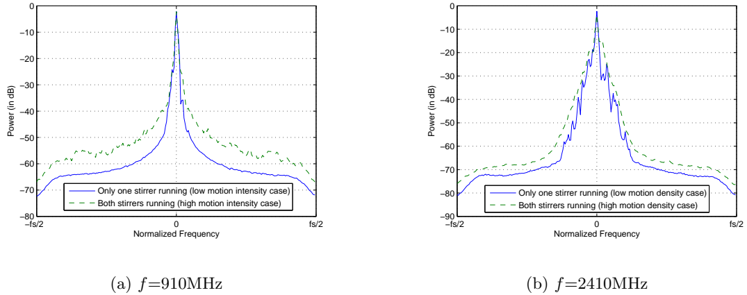
Figure 3.9 Impact of motion intensity on Doppler spectrum.
