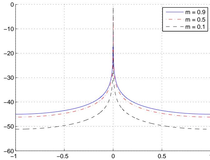
Figure 3.4 Doppler spectrum with moving objects case for different values of m .
