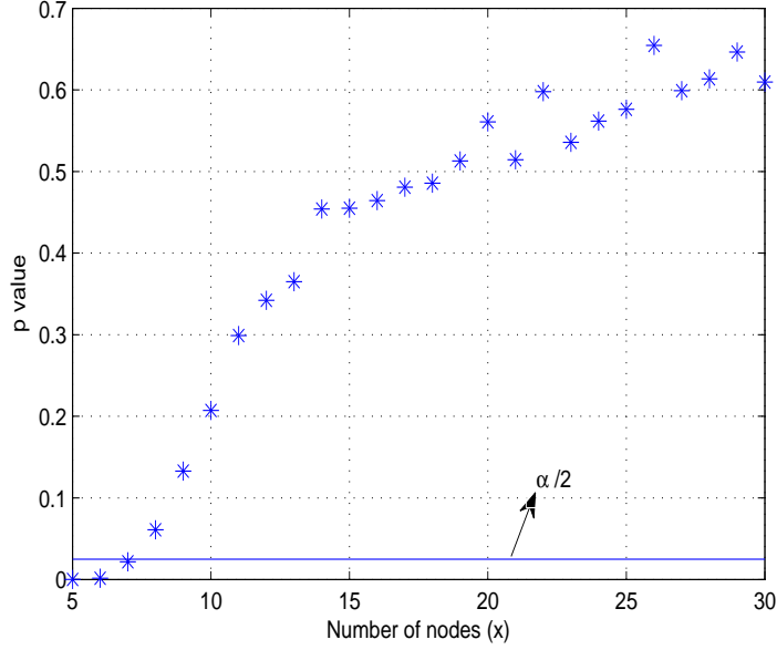
Figure 5.5 Results of KS test for the verification of Gaussianity assumption with Z_0=50\Omega and d_e=U[-1\Omega,1\Omega] .
