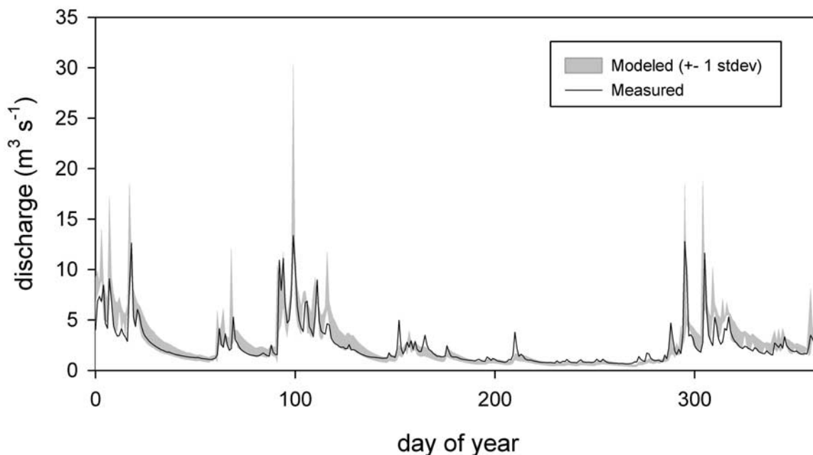
Figure 3. Measured and modeled discharge for the Upper Rye catchment, North Yorkshire, United Kingdom. The chart shows the mean and the \pm one standard deviation of the behavioral simulations.
