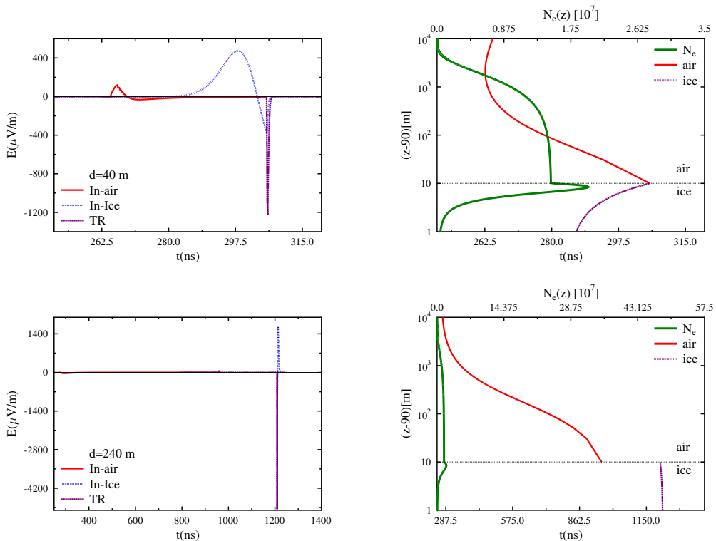
Figure 1. The electric field at different observer distances equal to, a) d = 40 m, b) d = 240 m. The figures on the right show the emission height, plotted as function of the observer time. The full red line gives the emission in air, the dotted purple line gives the transition radiation, and the dashed blue line gives the in-ice emission. For the figures on the right, the total number of particles is given by the full green line. Figure and caption taken from [1].
