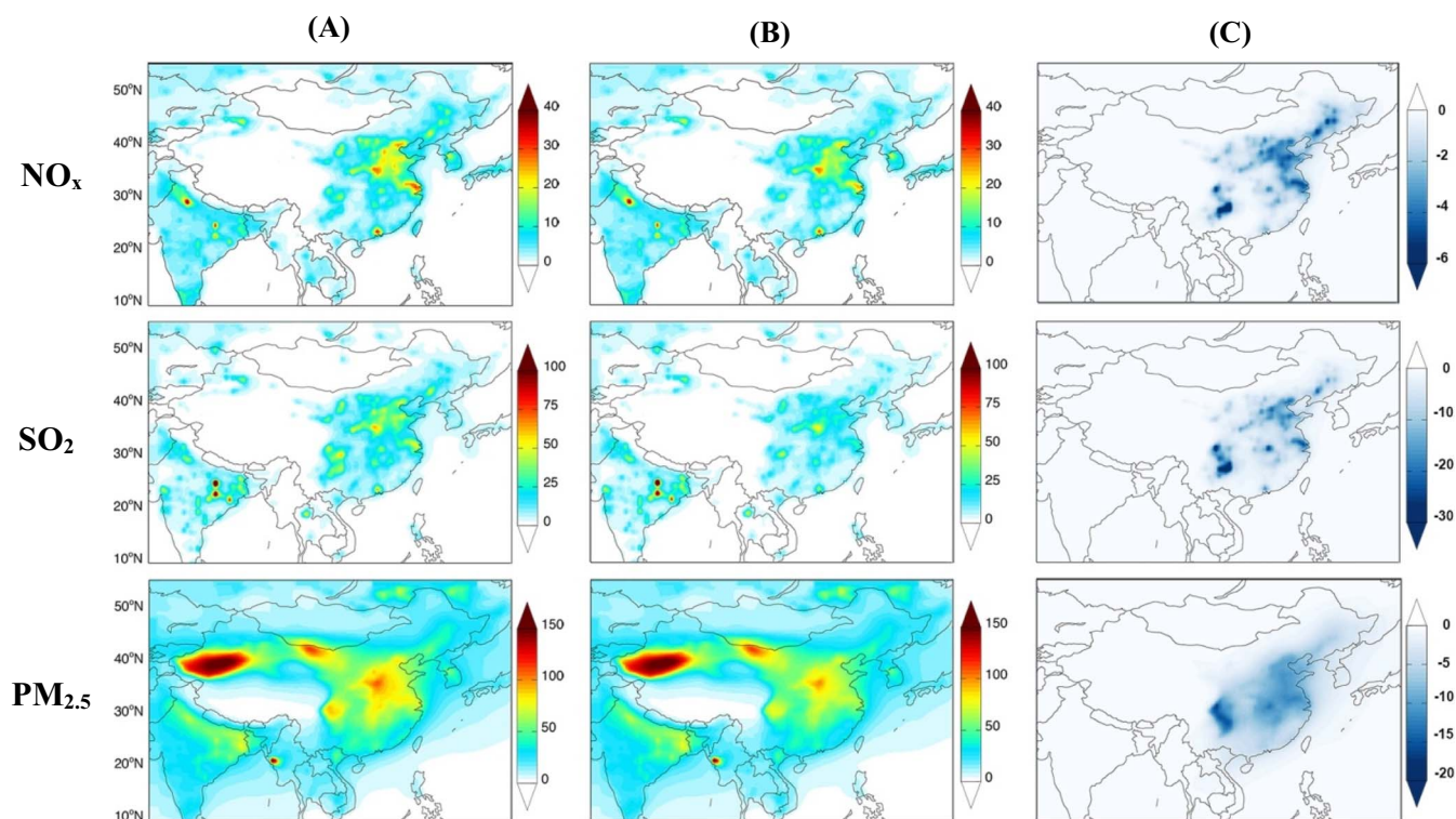
Fig. 1. Air concentrations of \text{NO}_x , \text{SO}_2 and \text{PM}_{2.5} in 2014 (base year) and 2020 (target year), and the reductions by SSSR. (A) presents the concentrations in 2014, which is the base year of this study. (B) presents the concentrations in 2020, which is the target year. (C) is the reductions of air concentrations by SSSR, which are calculated using the concentrations in 2020 minus those in 2014 in the same grid. The unit is \mu\text{g}/\text{m}^3 .
