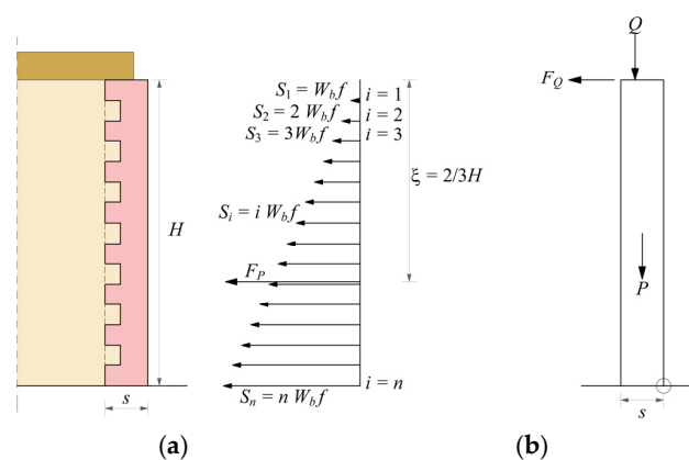
Figure 4. Frictional resistances transmitted to the façade wall by the shear walls (a) and the simply-supported horizontal diaphragm (b).
