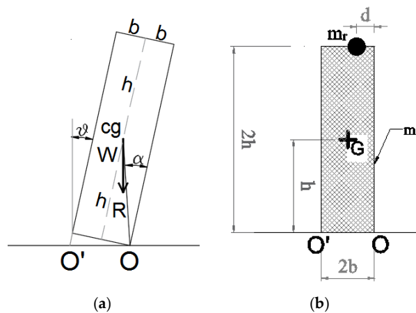
Figure 1. The rectangular free-standing rocking block of Housner's model (a) and the centroid G_c of the composed masonry block + the roof mass system with eccentricity d (b).
