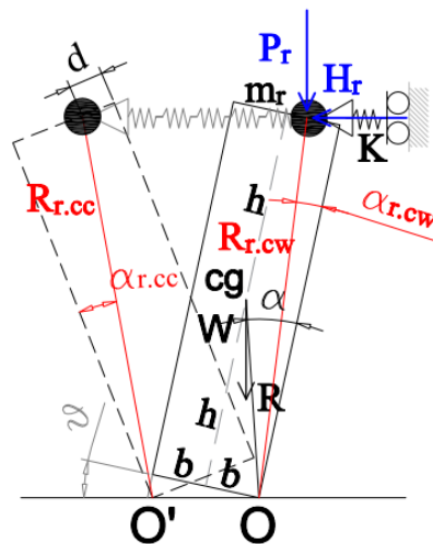
Figure 2. The rocking block with horizontal elastic restraint and roof mass.
