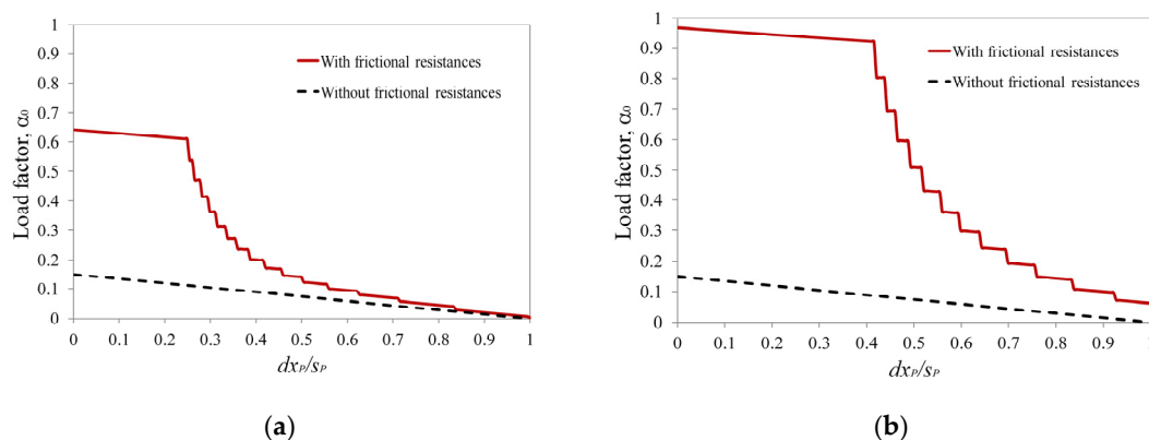
Figure 6. Influence of the frictional resistance due to interlocking between orthogonal walls after the hinge formation [13,49]. Pushover curves with unit aspect ratio h_b/l_b = 1/3 (a) and h_b/l_b = 1/5 (b).
