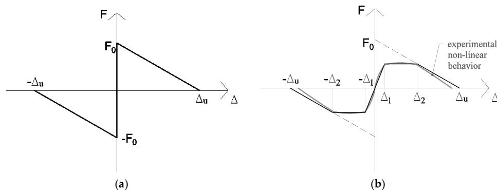
Figure 5. Force-displacement law for the rocking block: ideal model (a); model with imperfections (b).
