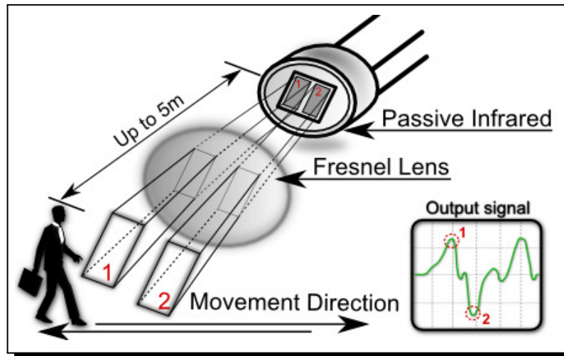
Figure 2. PIR motion sensor operation
