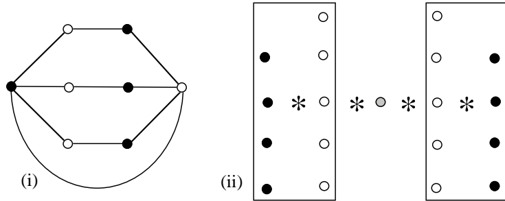
Figure 1: (i) exception for Theorem 3, (ii) the graph H_5 .
