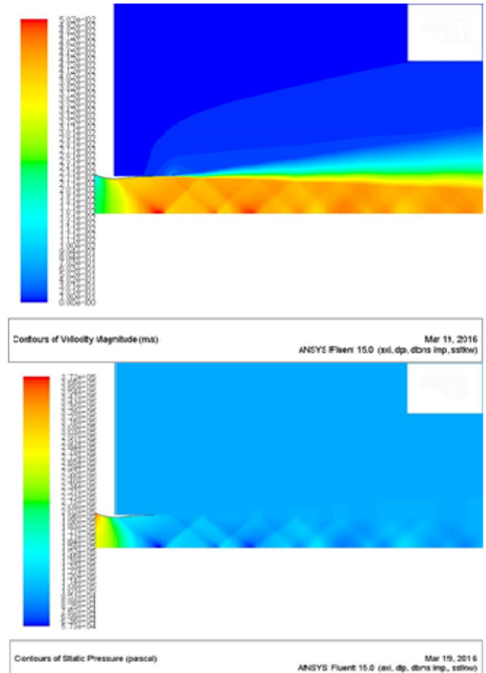
Fig.4 Contours of Velocity Magnitude & Static Pressure for nozzle 2
