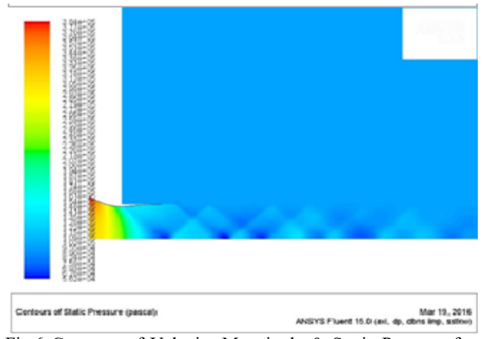
Fig.6 Contours of Velocity Magnitude & Static Pressure for nozzle 4
