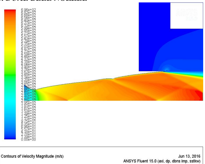
Fig.7 Contours of Velocity Magnitude for dual bell nozzle
