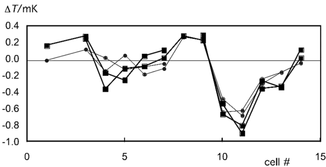
Fig. 2. Graphical representation of the corrected data \Delta T = (T_{\text{meas,ac}} - T_{\text{KCRV,ac}}) from Table 3 and the uncorrected data \Delta T = \Delta T_{\text{original}} from Table 2, for cells #1 to #15 and for thermometer sets #1 and #2. Gray dots and lines: uncorrected differences. Black squares and lines: isotopic-corrected differences.
