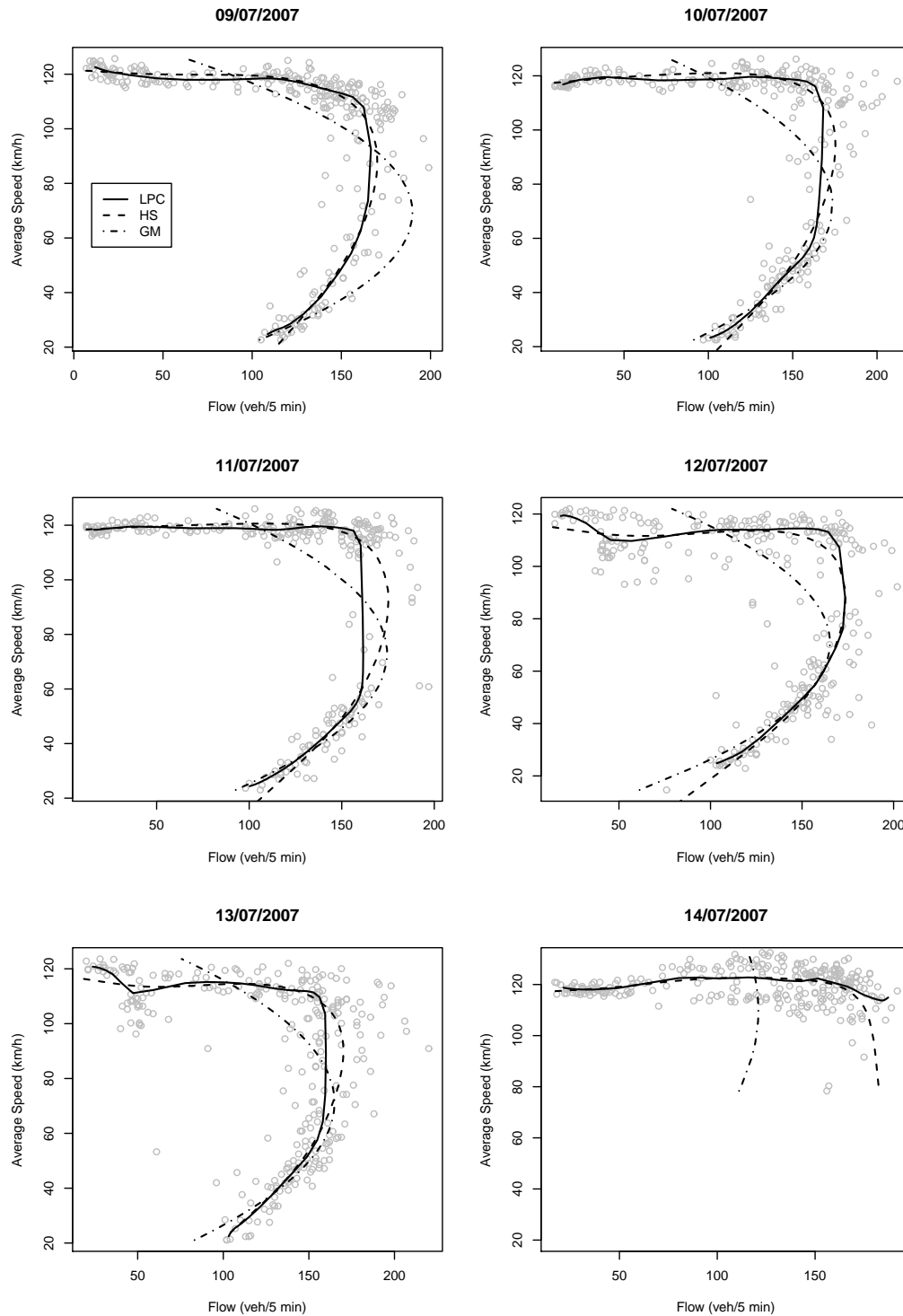
Figure 5: Speed-flow data from VDS 716450 with local principal curve, HS principal curve, and Greenshields curve, for six consecutive weekdays starting 9th of July 2007.
