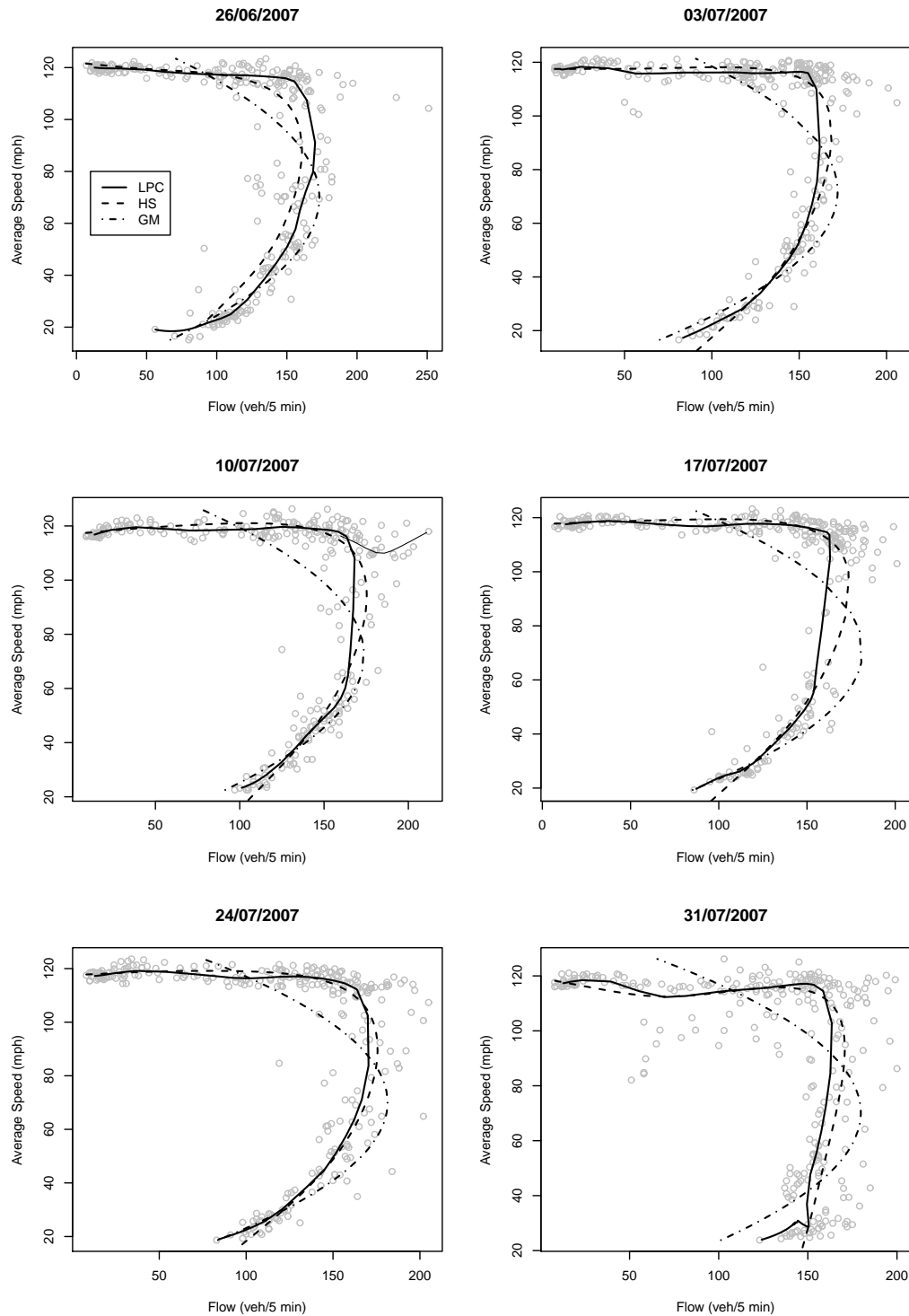
Figure 6: Speed-flow data from VDS 716450 with local principal curve, HS principal curve, and Greenshields curve, for six consecutive Tuesdays starting 26th of June 2007.
