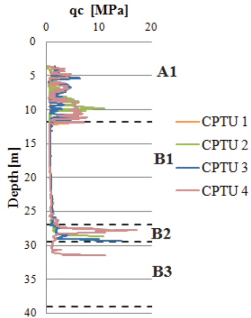
Fig. 6 – Tip resistance profile.
