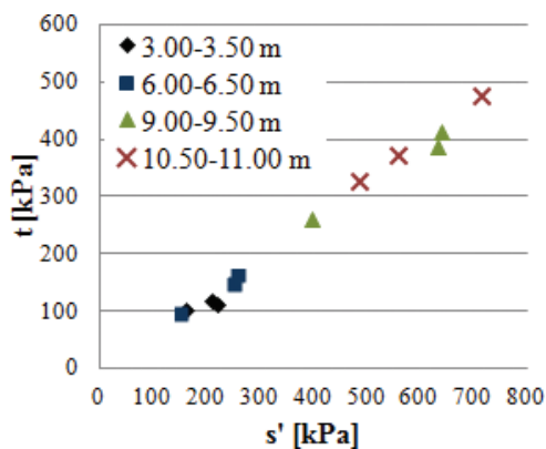
Fig. 8 – Failure stresses of A1 layer.
