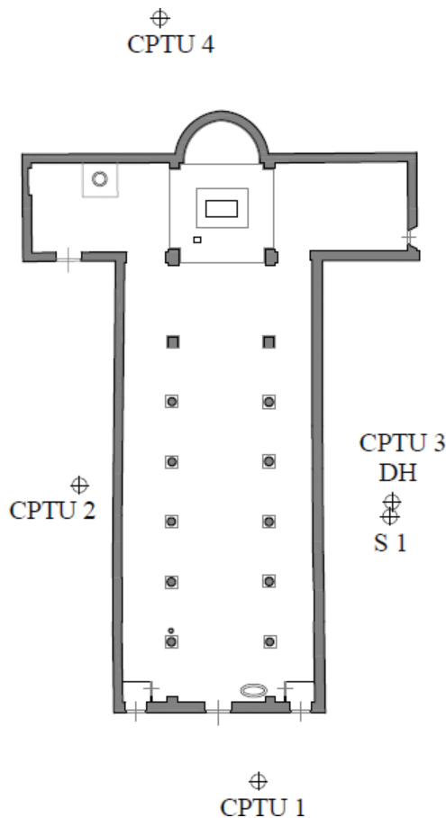
Fig. 5 – Plan of geotechnical investigations.
