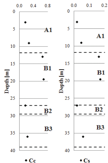
Fig. 10 – Compressibility parameters.
