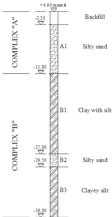
Fig. 7 – Stratigraphic model.
