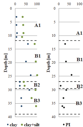
Fig. 9 – Soil fractions and plastic index profiles.
